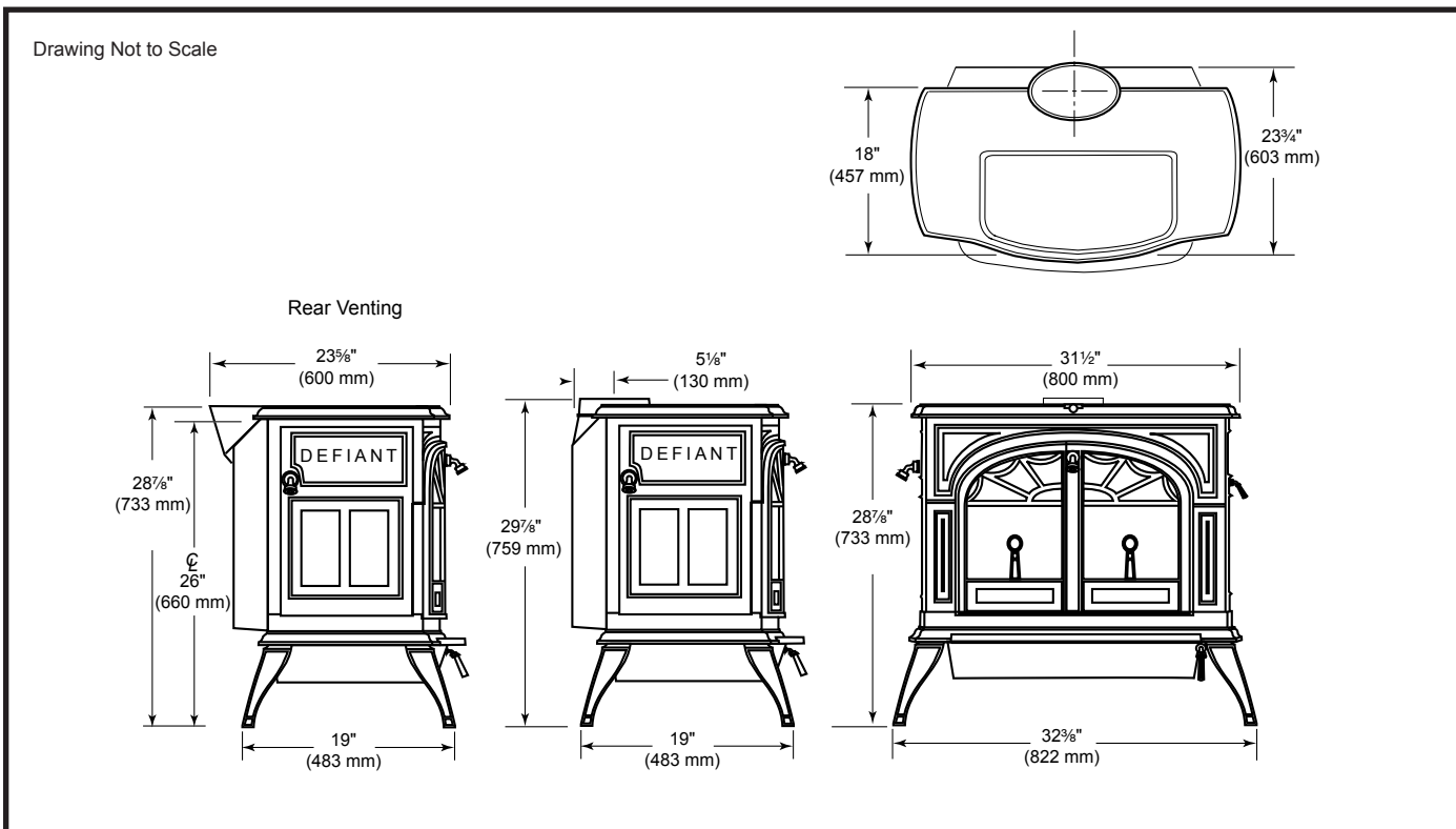
Fig. 1 Defiant 1975 dimensions.
